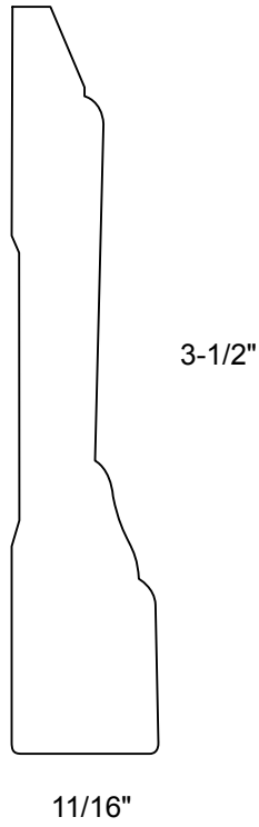
331 - Casing
