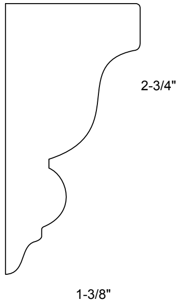
9083 Crown/Header
